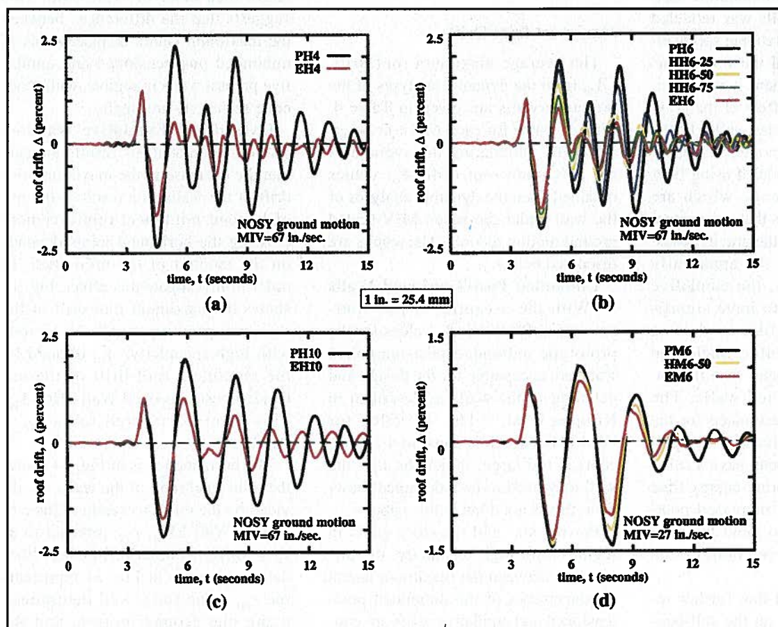
Fig. 13. Roof drift time history: (a) four-story, high seismicity; (b) six-story, high seismicity; (c) ten-story, high seismicity; (d) six-story, moderate seismicity.
