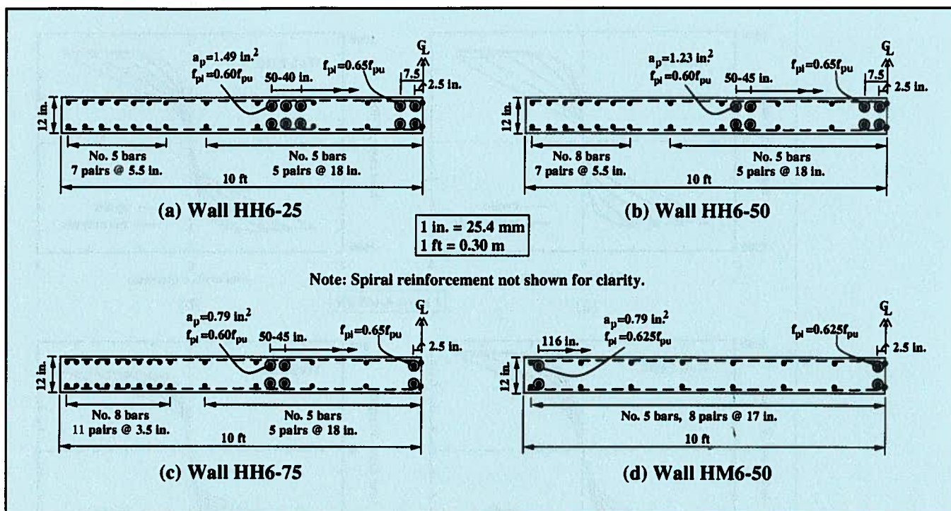
Fig. 7. Cross section (half wall length near base) of hybrid walls: (a) HH6-25; (b) HH6-50; (c) HH6-75; (d) HM6-50.
