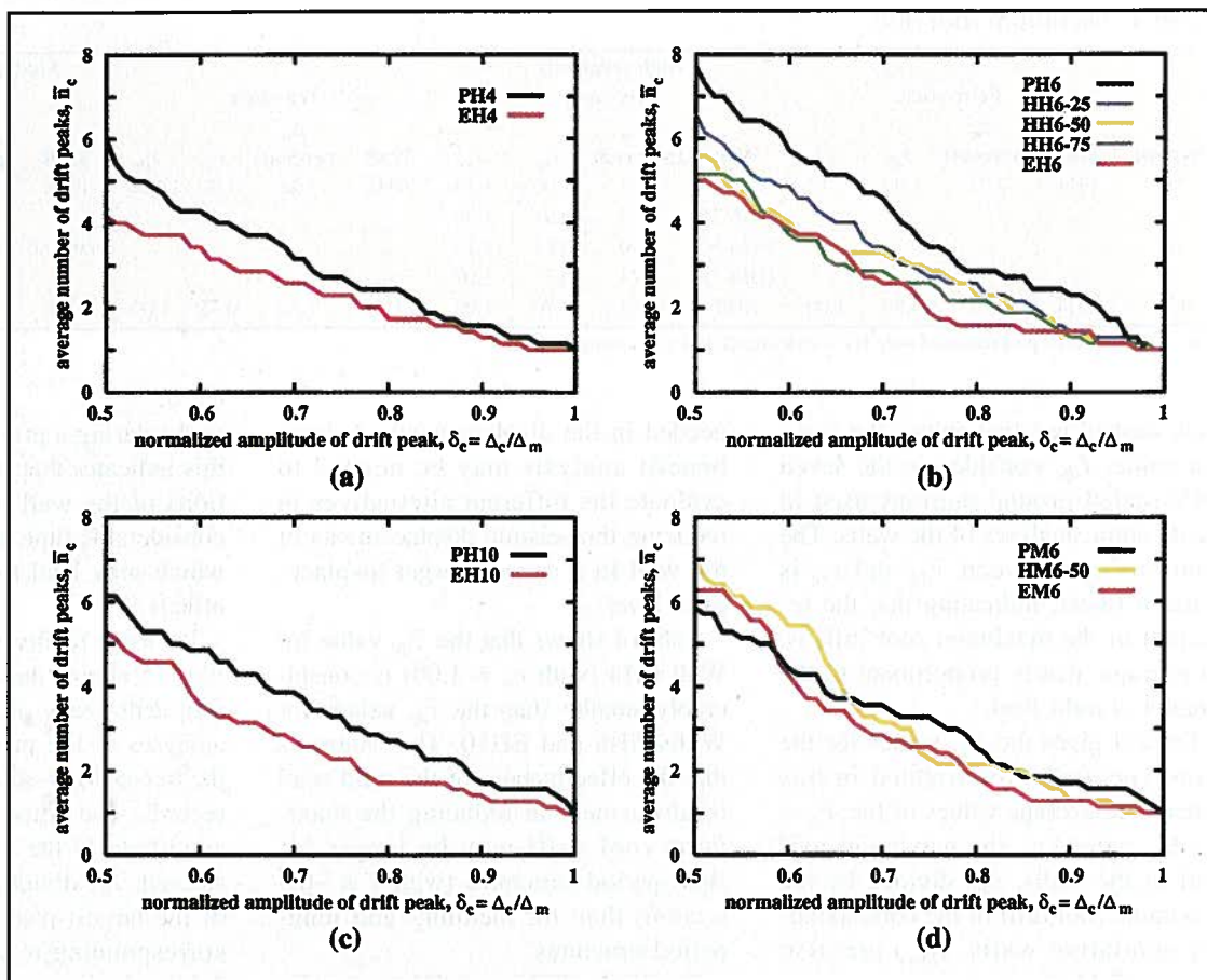
Fig. 15. \bar{n}_c versus \delta_c : (a) four-story, high seismicity; (b) six-story, high seismicity; (c) ten-story, high seismicity; (d) six-story, moderate seismicity.
